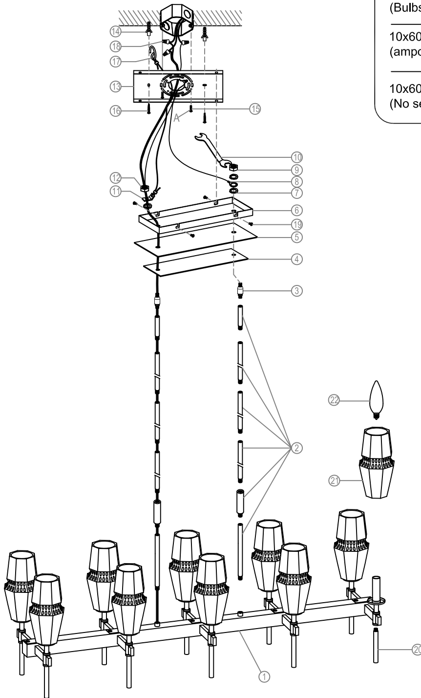
Wire connection
