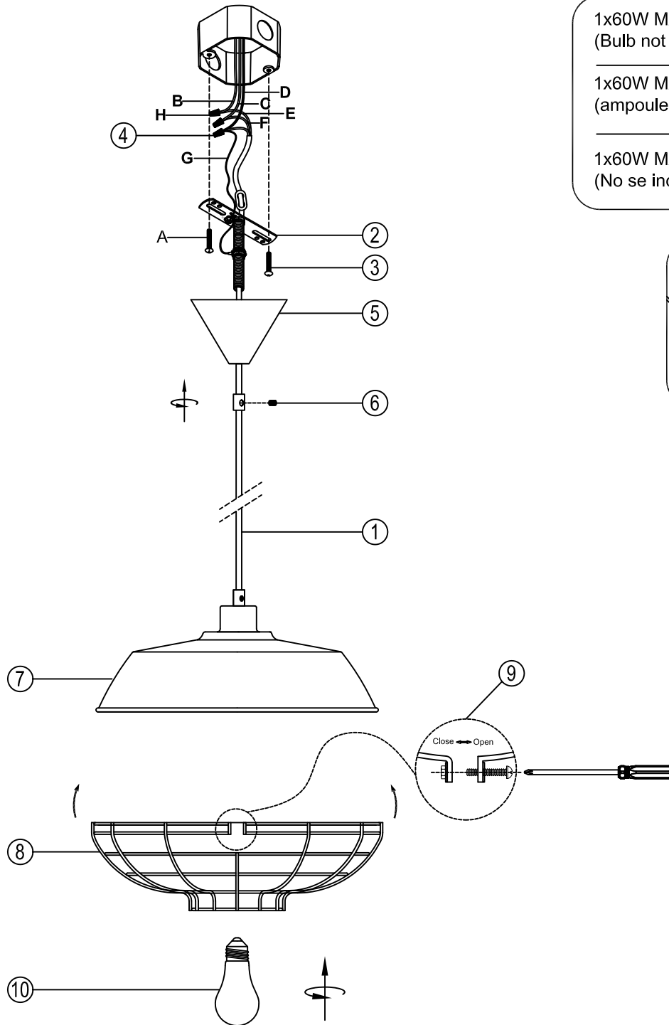
Wire connection
