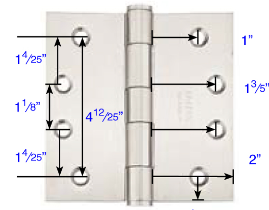
4 1/2" x 4 1/2" Residential Duty Plain Bearing with Square Corners
