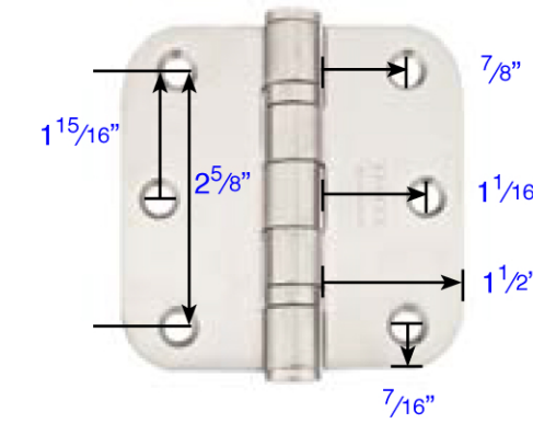
3 1/2" x 3 1/2" Heavy Duty Ball Bearing with 1/4" Radius Corners
