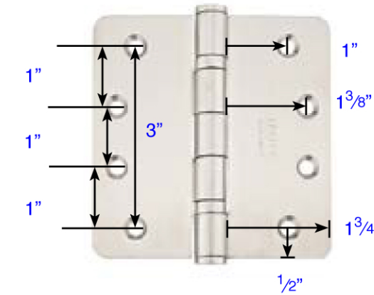
4" x 4" Heavy Duty Ball Bearing with 1/4" Radius Corners
