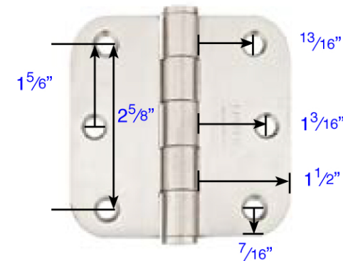
3 1/2" x 3 1/2" Heavy Duty Plain Bearing with 1/4" Radius Corners
