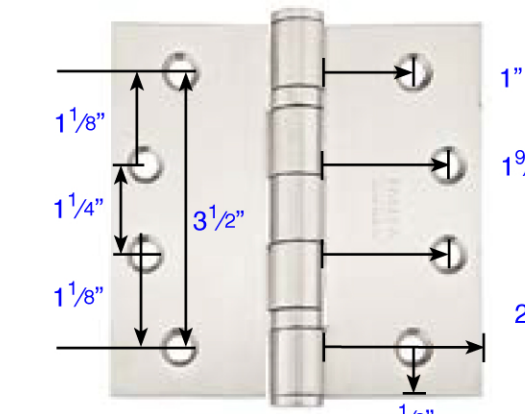
4 1/2" x 4 1/2" Residential Duty Ball Bearing with Square Corners
