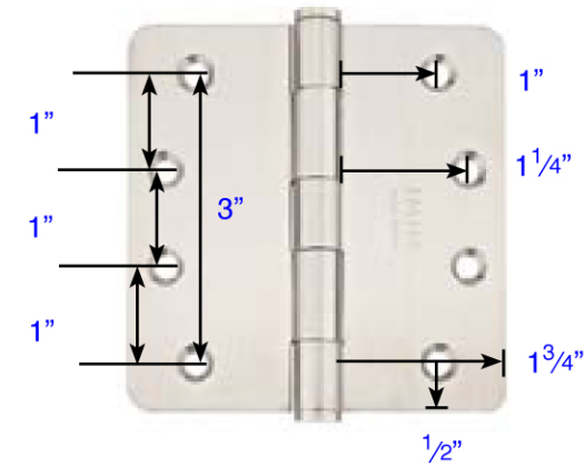
4" x 4" Heavy Duty Plain Bearing with 1/4" Radius Corners
