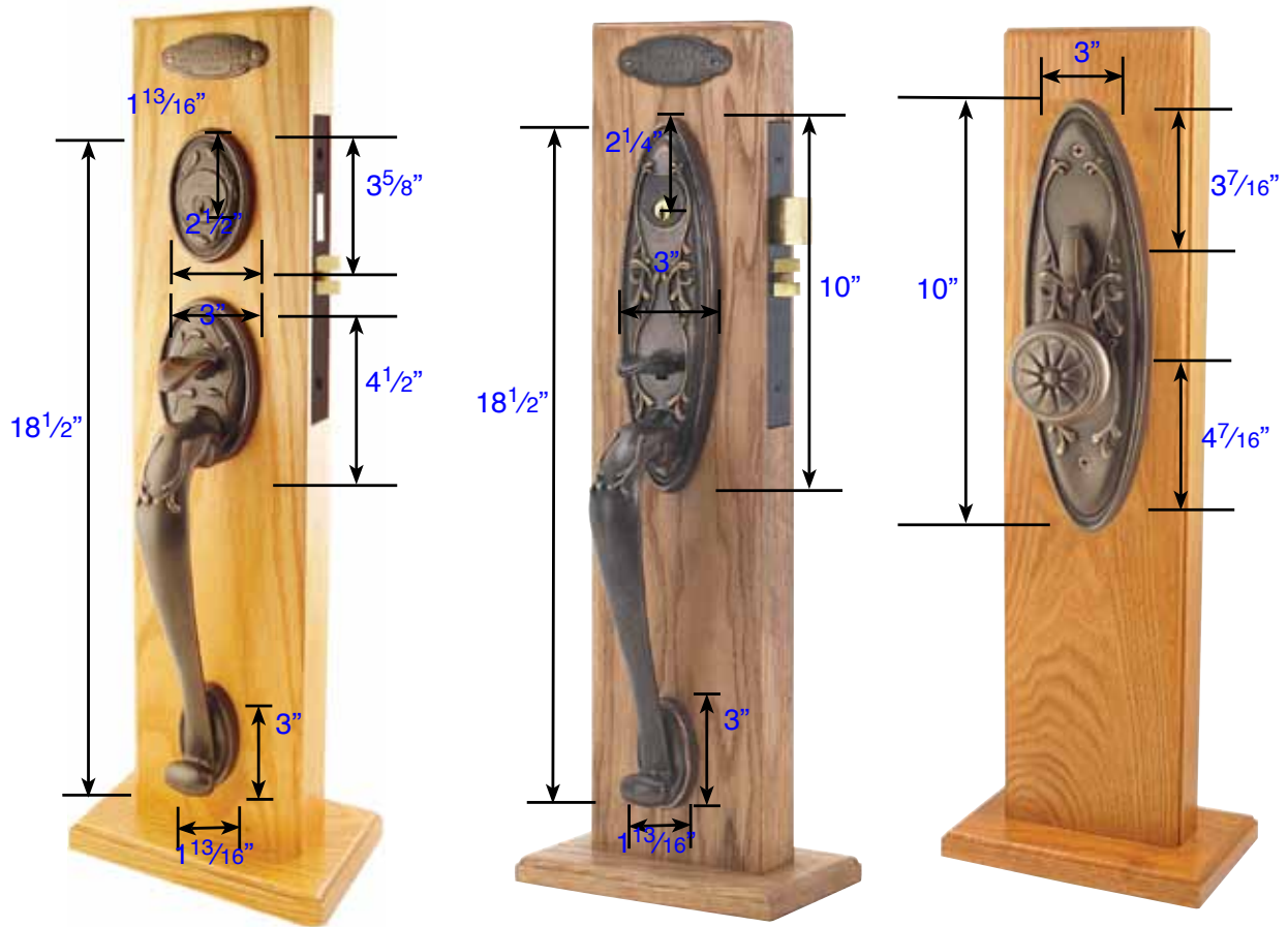
Naples UL Mortise Entryset Part # UL 3334
