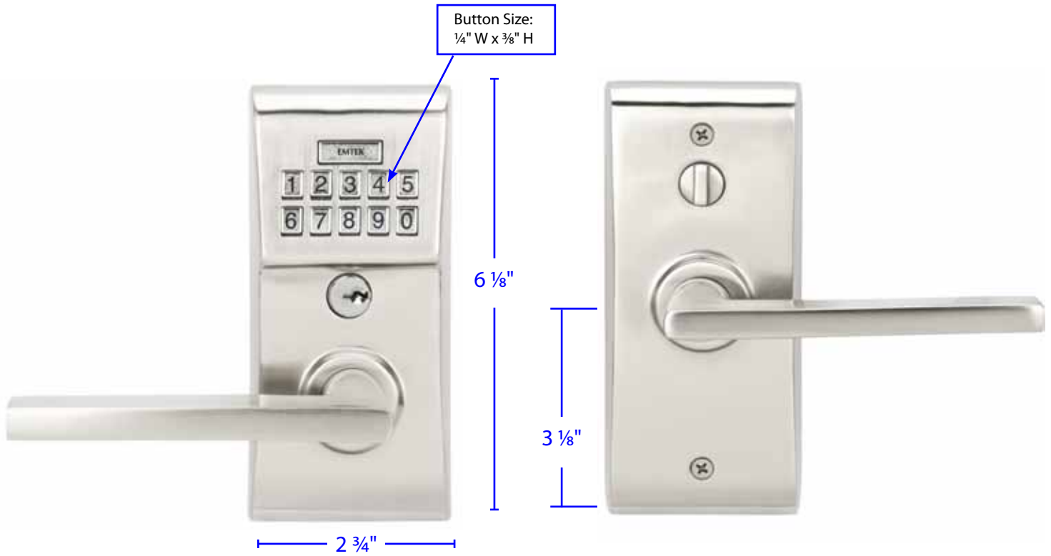
Exterior Projection: 3"
