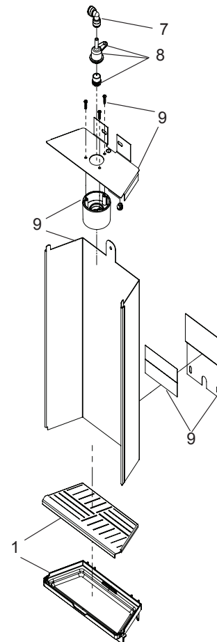
Alcove Assembly
