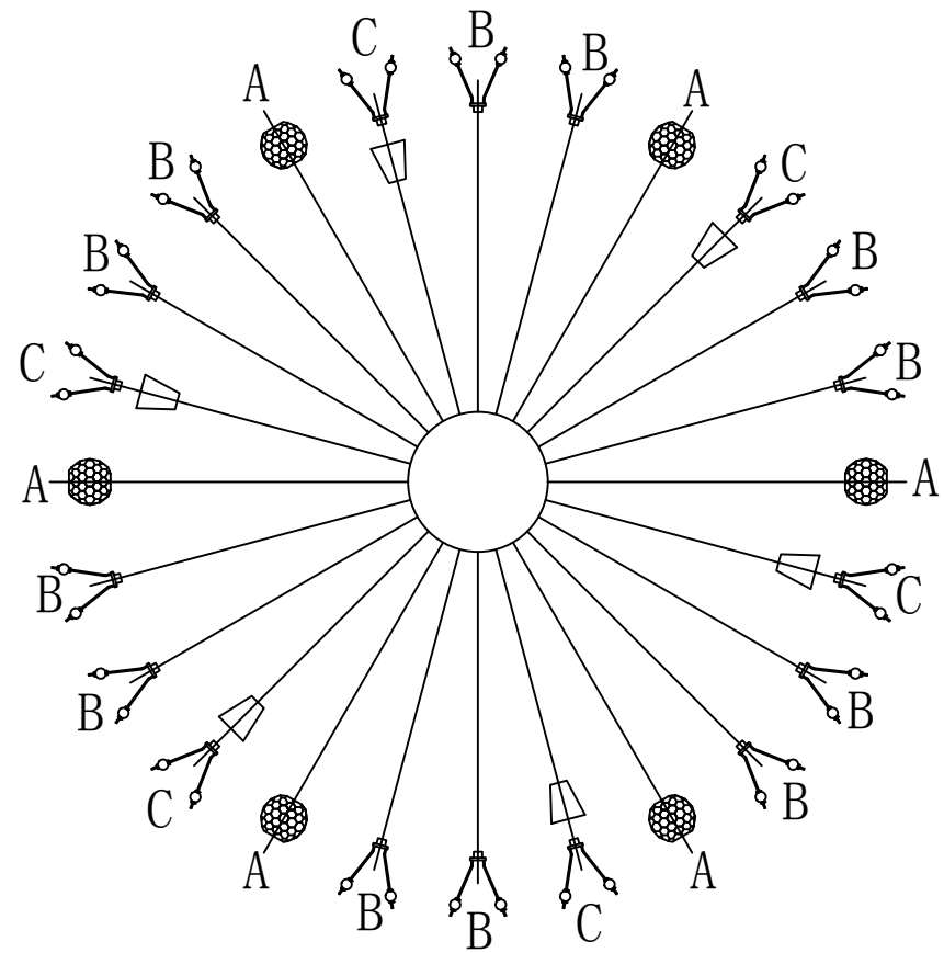
layer 3 Installation diagram
