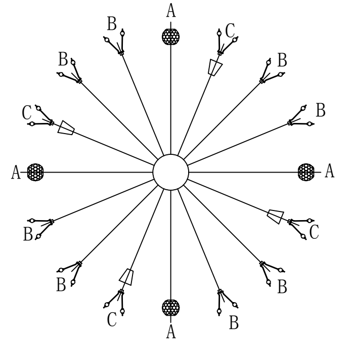
layer 5 Installation diagram
