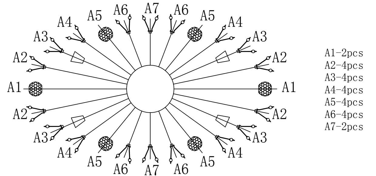
layer A Installation diagram
