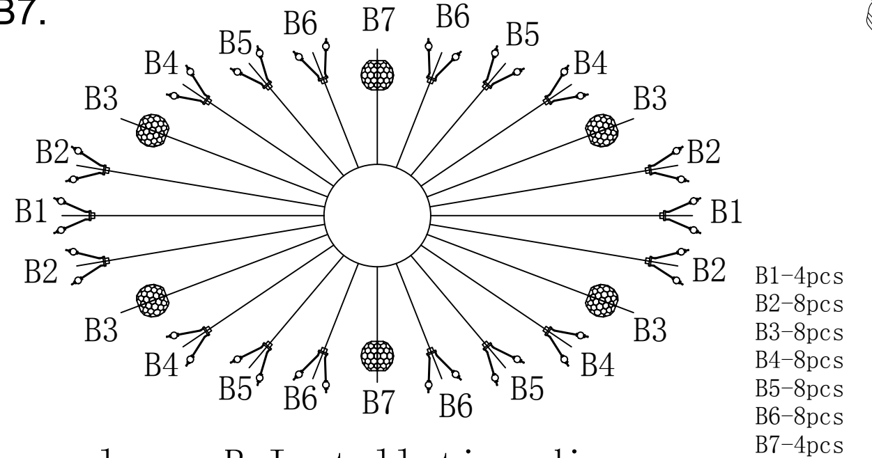
layer B Installation diagram
