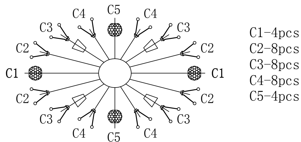
layer C Installation diagram
