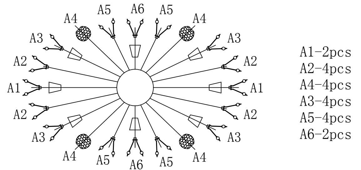
layer A Installation diagram
