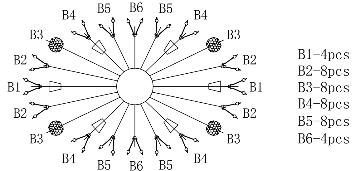
layer B Installation diagram
