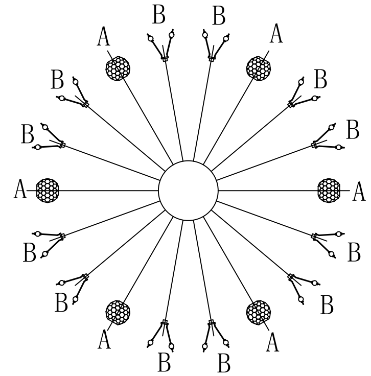
layer 2 Installation diagram
