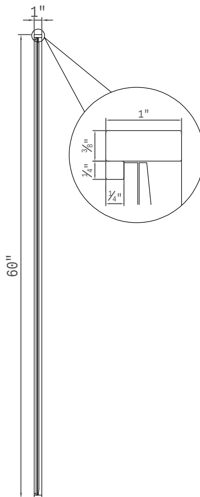
Side view
