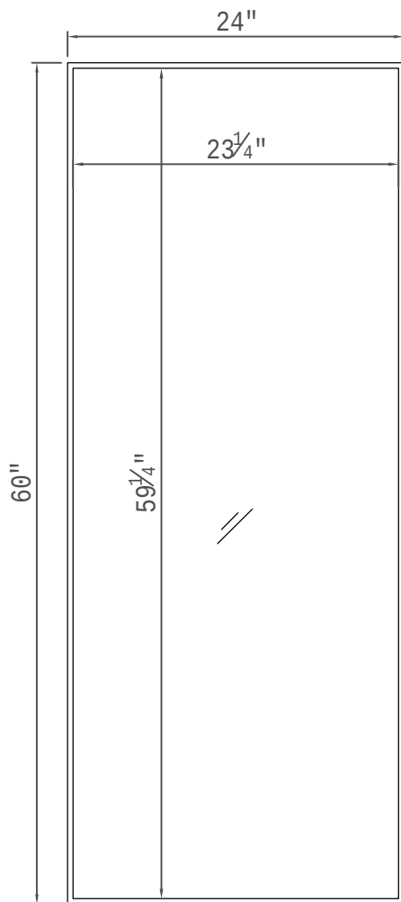
Front view
