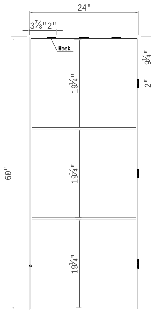
Back view
