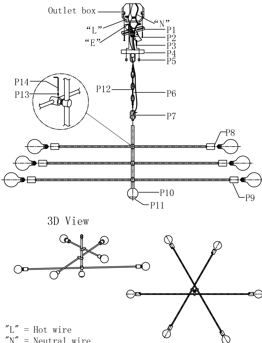
Bottom View 1:4
