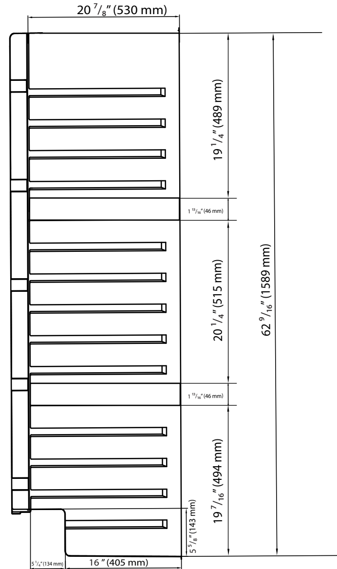
Side View
