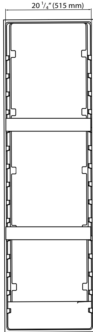
Front View
