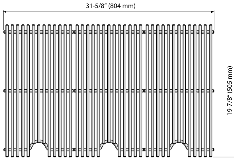
Grilling Surface
