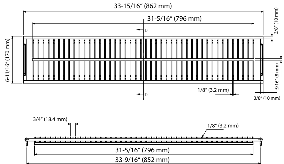
Warming Rack
