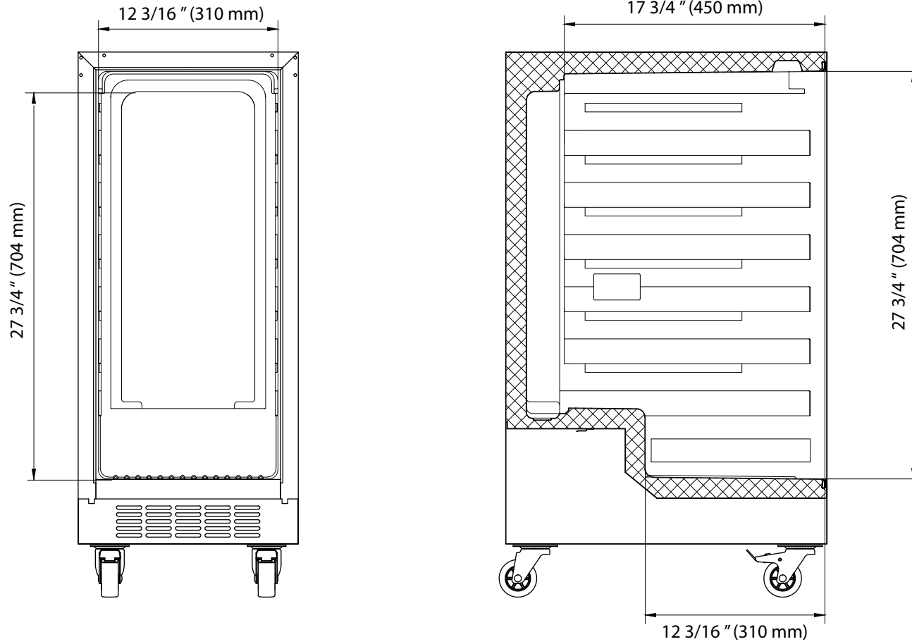
Front View
