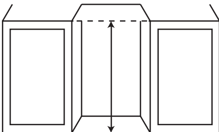
Cutout Height: 25 3/8"
