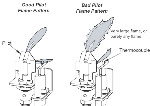
Figure 21 - Pilot Flame Pattern
