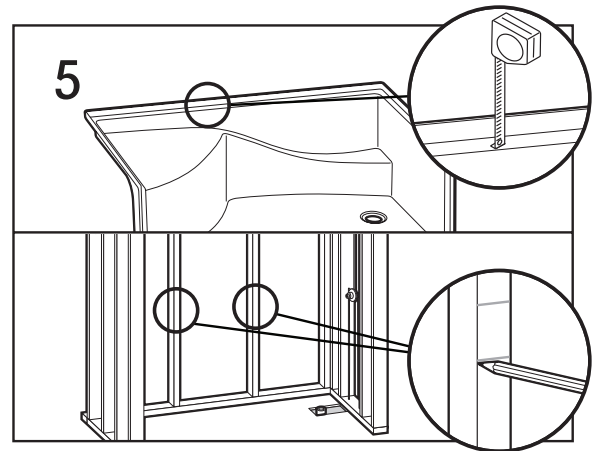
Measure the distance between the top of the back horizontal flange and the bottom of the pan ledge, approximately 1-1/2". Mark this dimension on the back studs (or wall), below the first mark.
