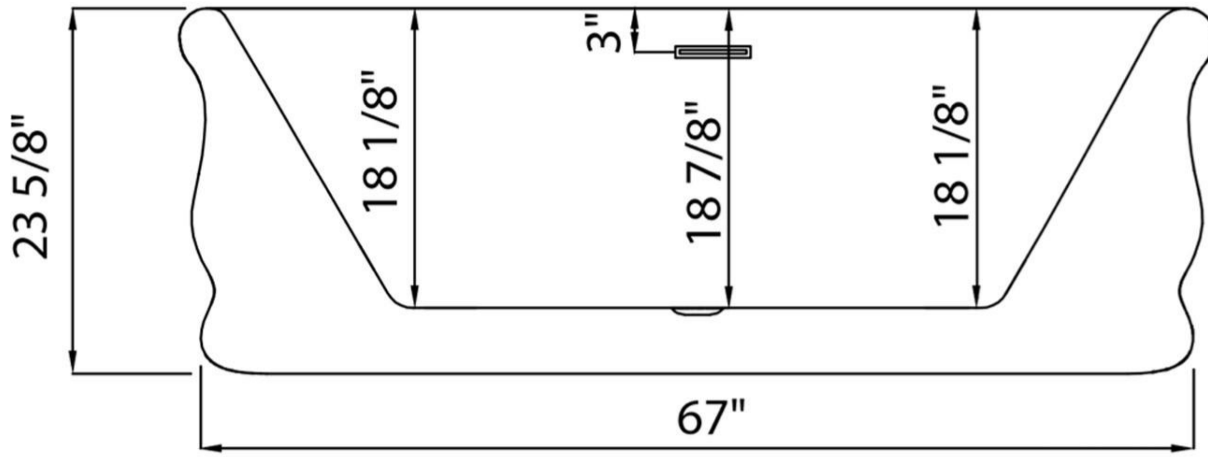
FRONT VIEW
