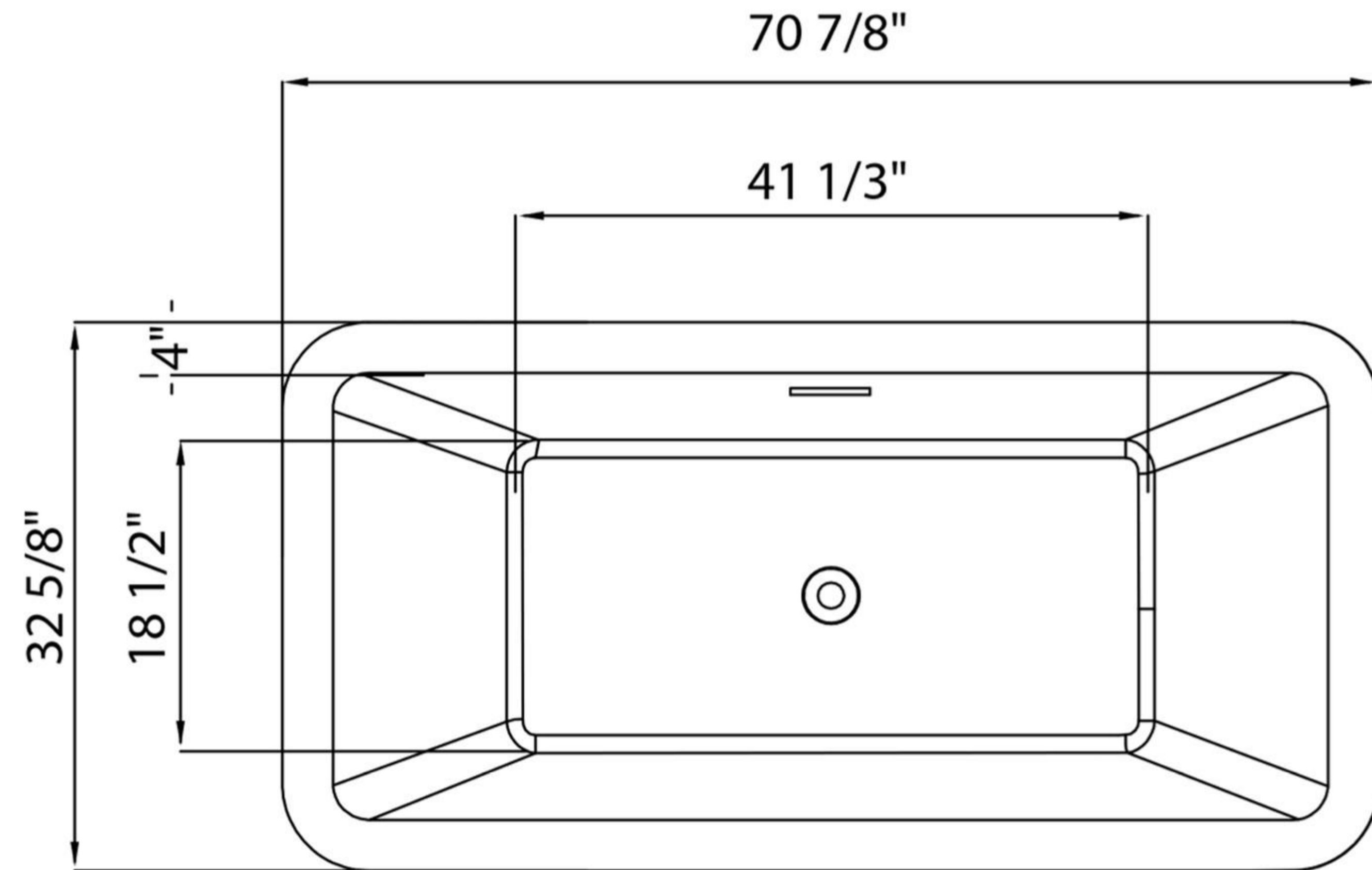
TOP VIEW
