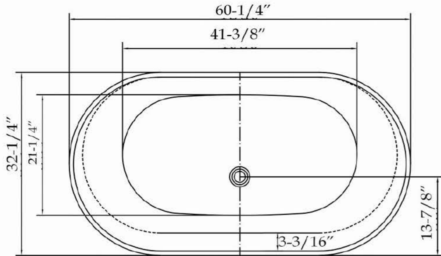
TOP VIEW
