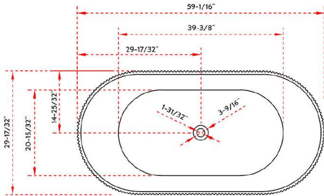
TOP VIEW
