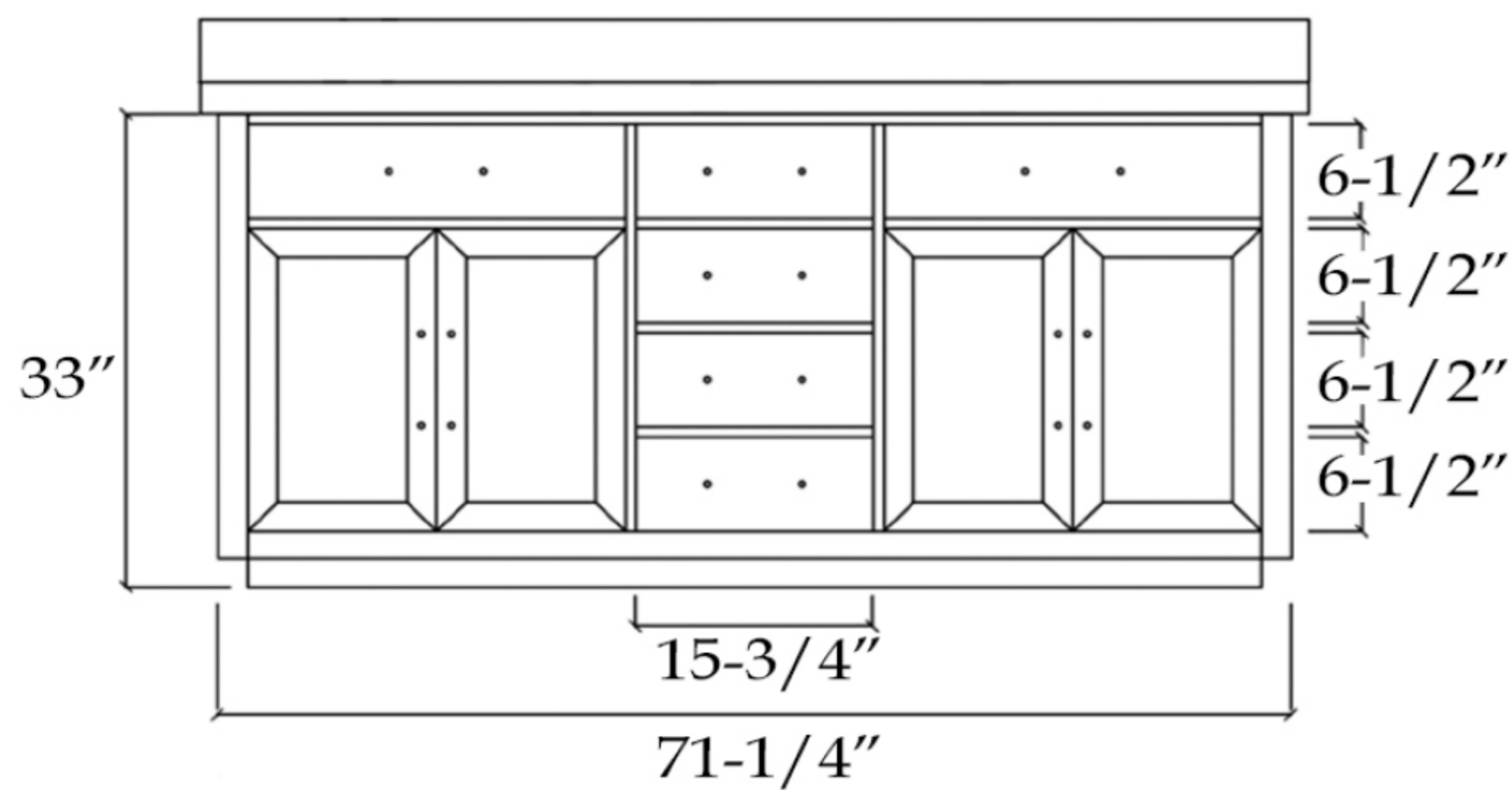
FRONT VIEW
