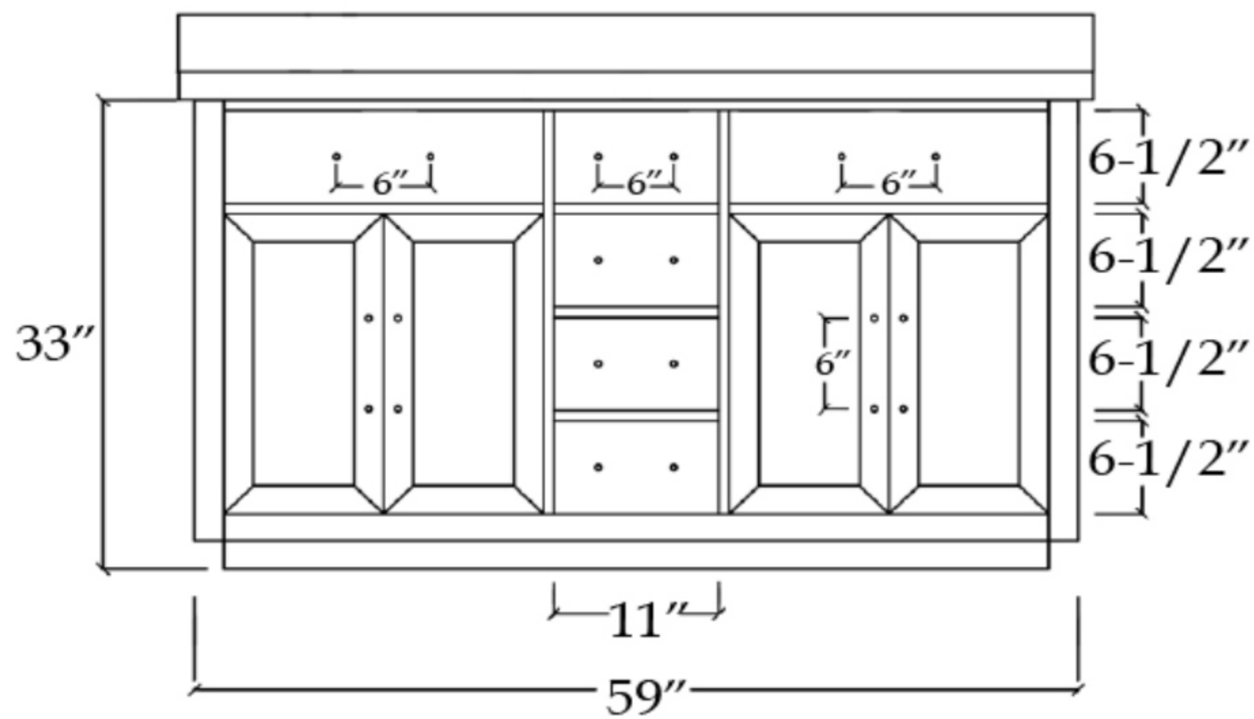
FRONT VIEW
