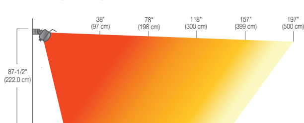
SIDE PROFILE
