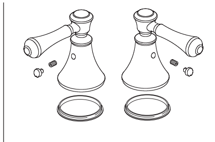
H697▲ Handle Assembly (not included) Ensamble de la manija (no incluido) Manette (non inclus)
