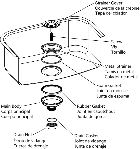
Insert metal strainer into drain hole with foam gasket attached. Install rubber gasket and main body underneath the sink
