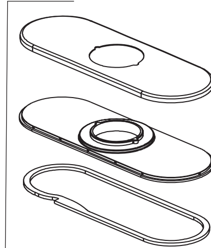
RP101774▲ (Escutcheon optional, included) Escutcheon with Baseplate (3 Hole) Chapetón y Empaque (3 agujeros) Boîtier et Joint (3 trous)
