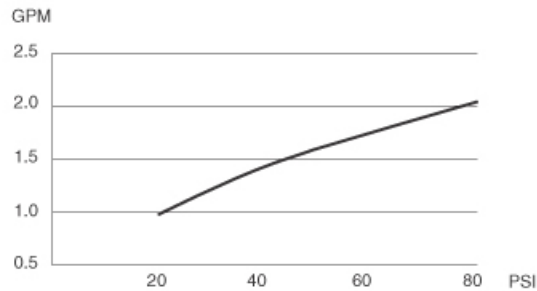
SHOWERHEAD FLOW RATE CHART
