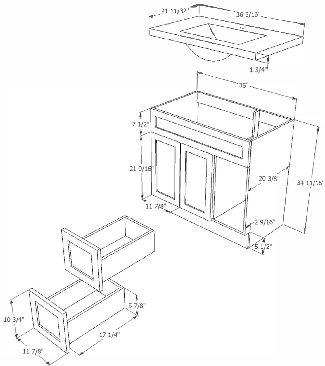
DAISY Collection 36" Freestanding Vanity
