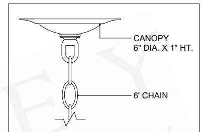
CANOPY DETAIL
