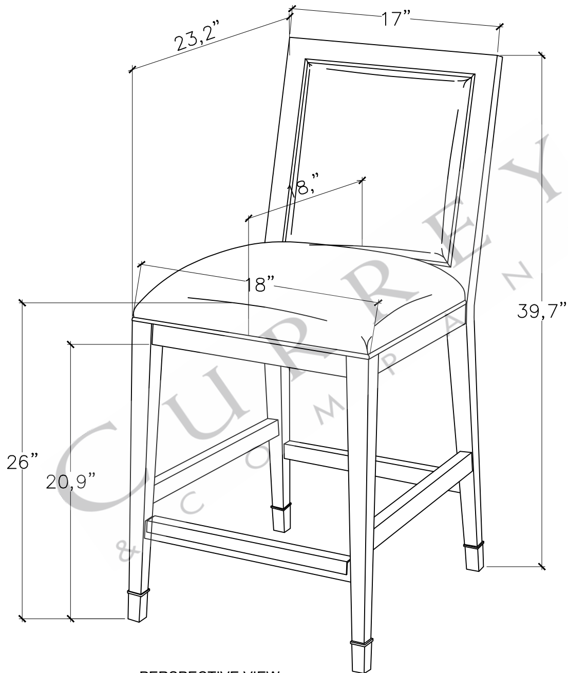
PERSPECTIVE VIEW
