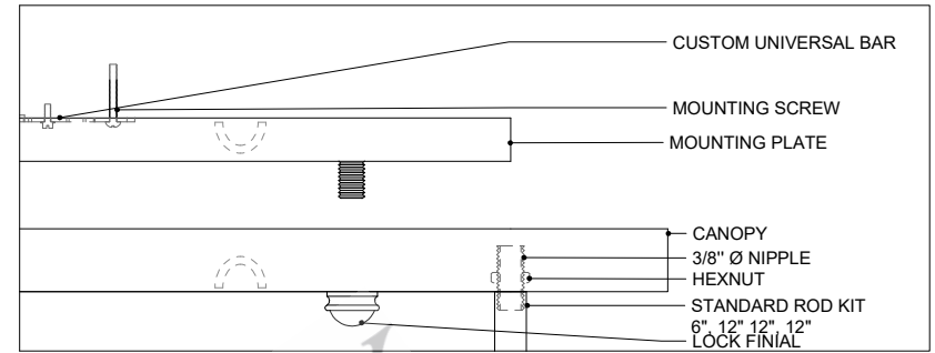
CANOPY DETAIL
