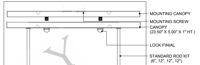
CANOPY DETAIL
