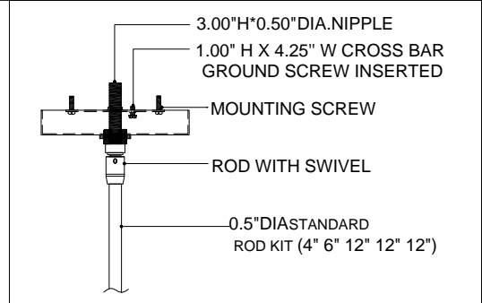
CANOPY DETAIL
