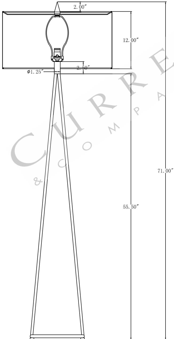
FRONT VIEW
