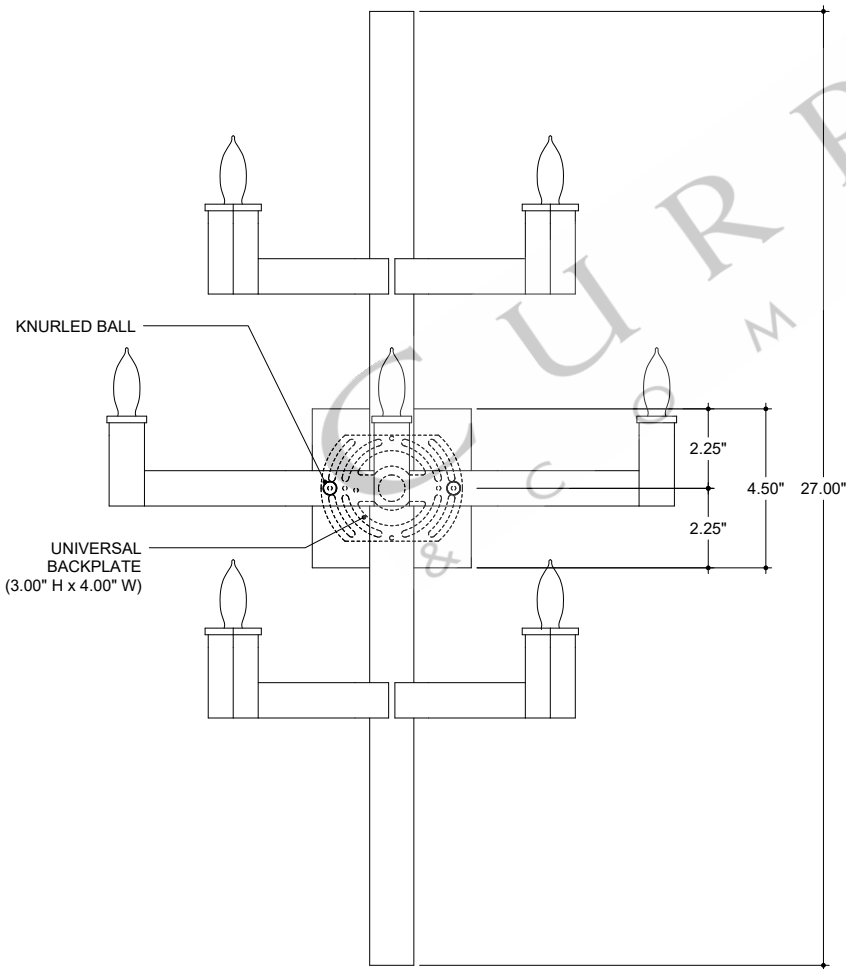
FRONT VIEW
