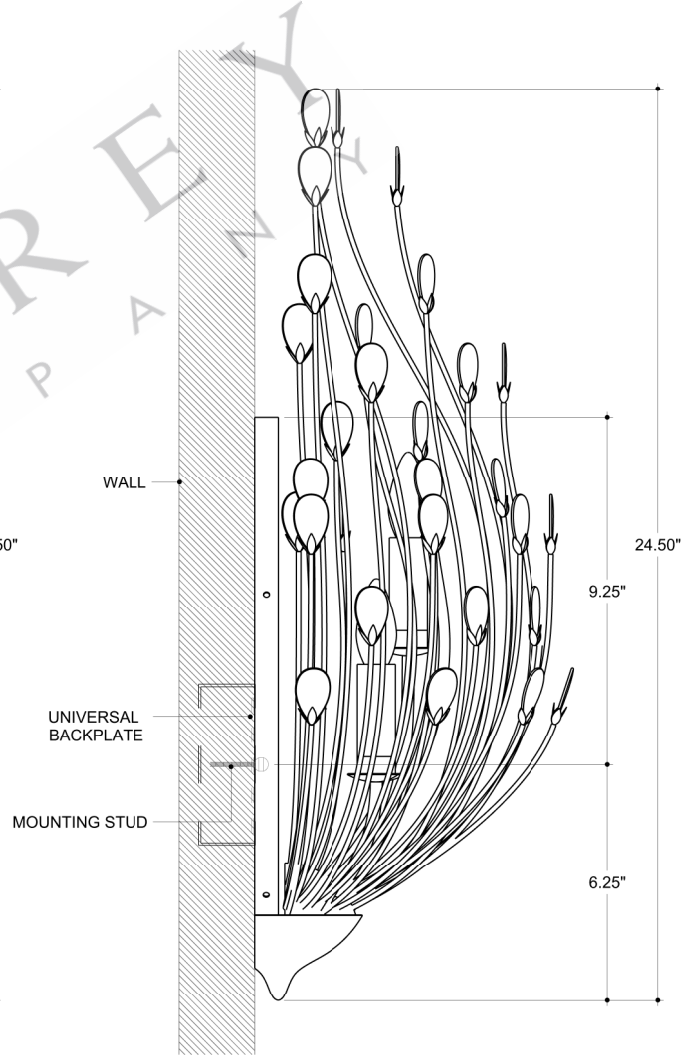
SIDE VIEW
