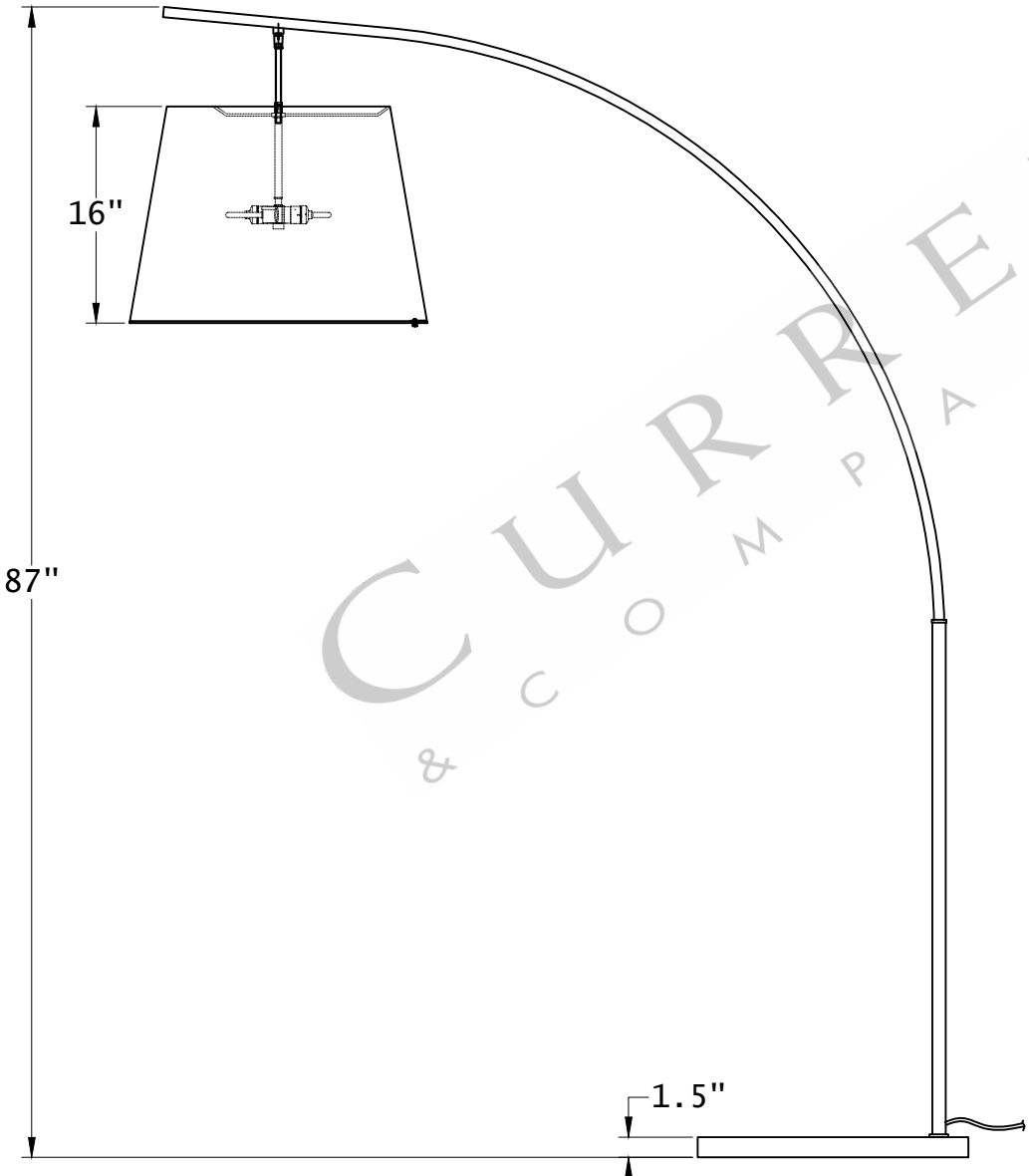
SIDE VIEW
