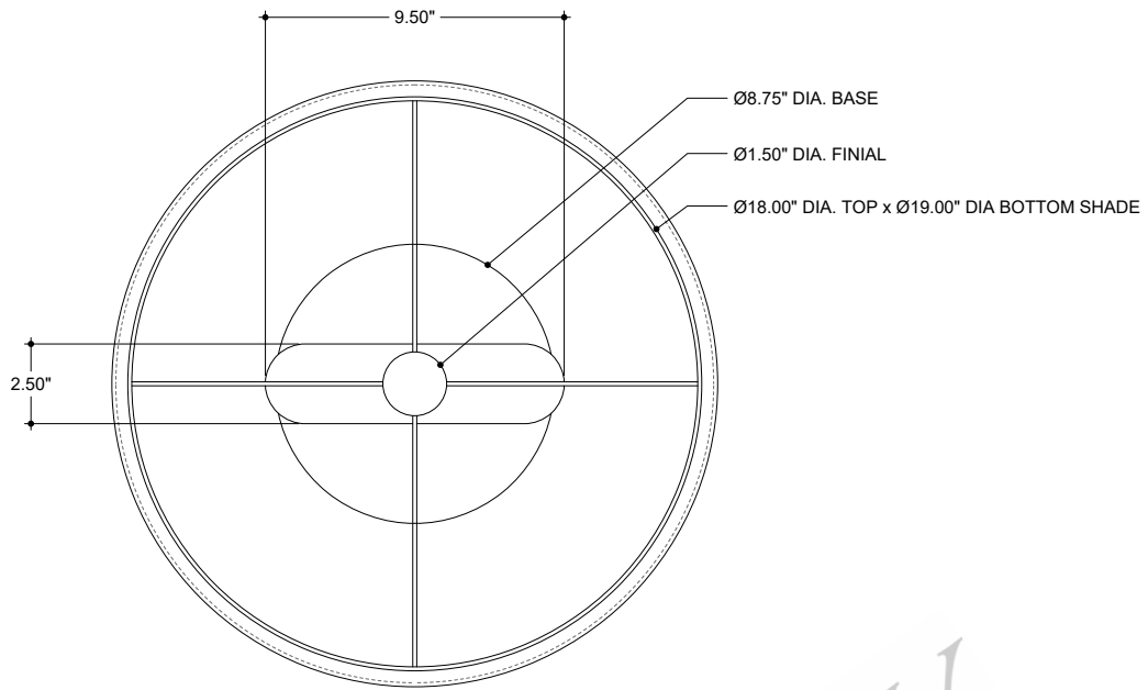
TOP VIEW
