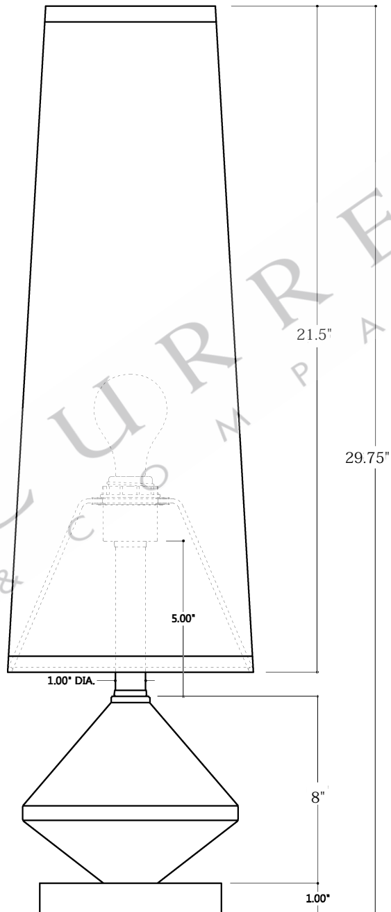
FRONT VIEW
