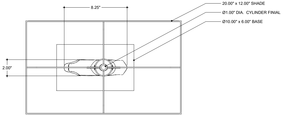
TOP VIEW
