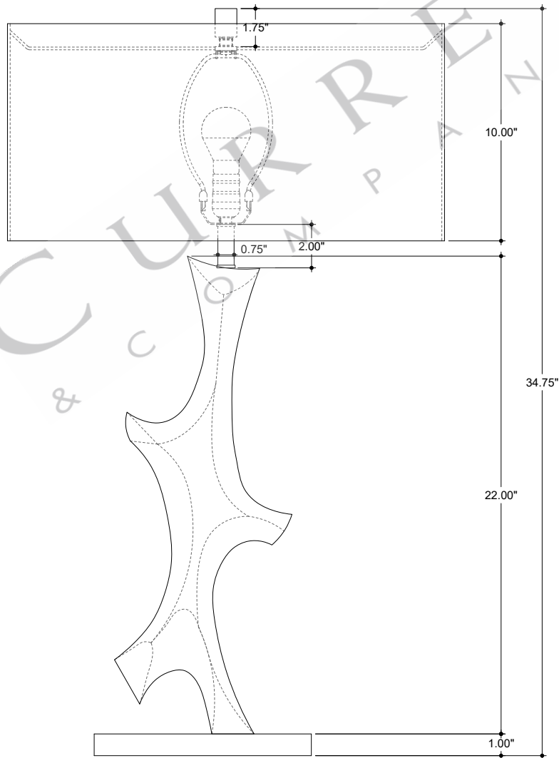
FRONT VIEW
