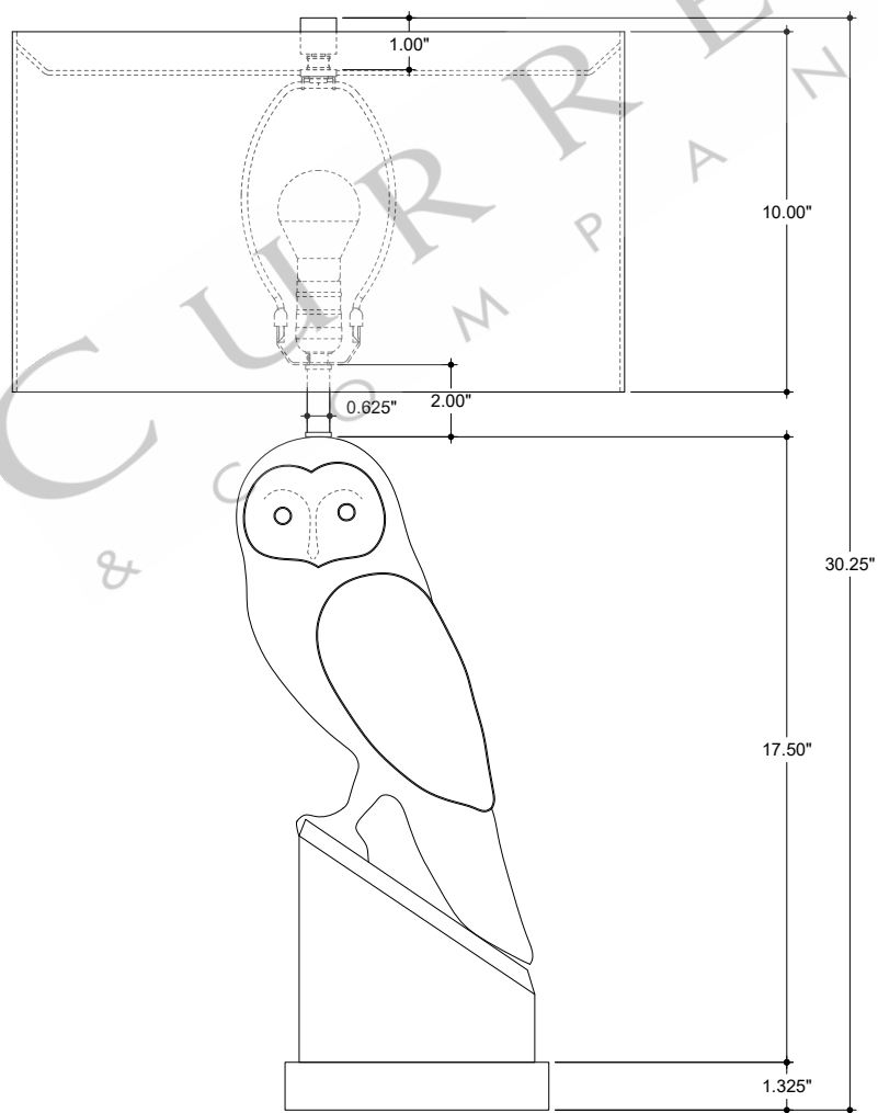
FRONT VIEW
