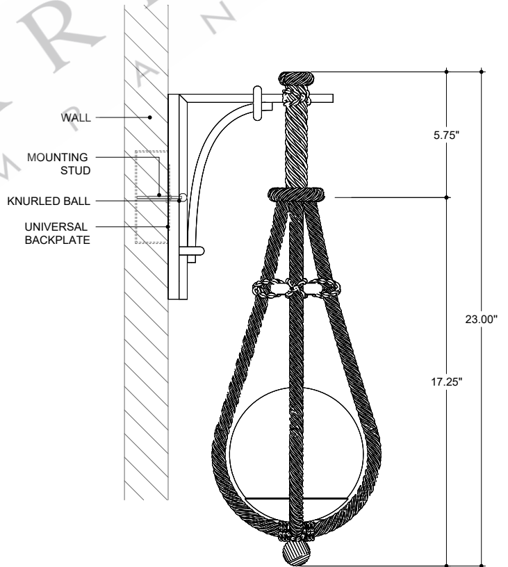
SIDE VIEW
