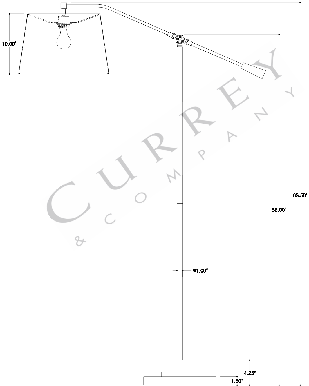
FRONT VIEW
