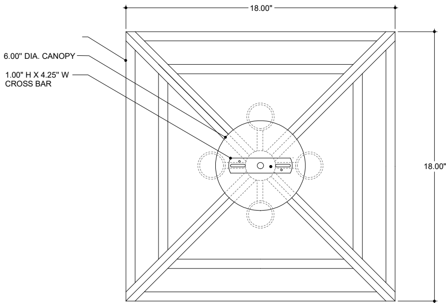
CANOPY DETAIL
