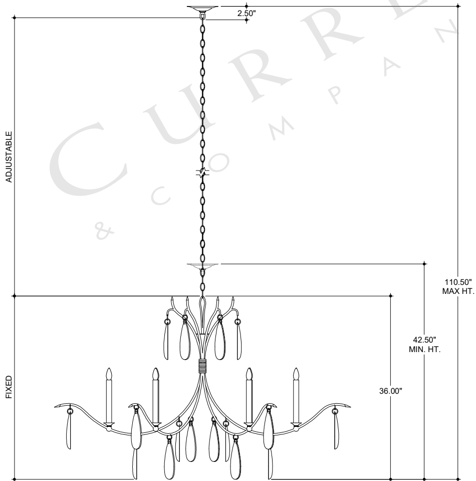
FRONT VIEW
