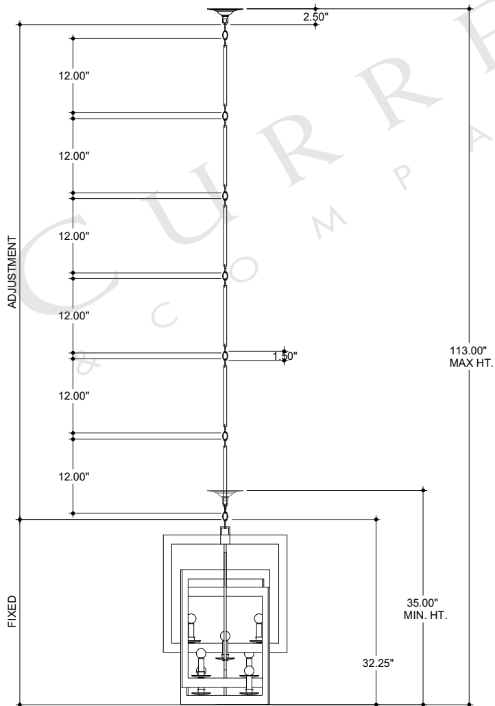
FRONT VIEW
