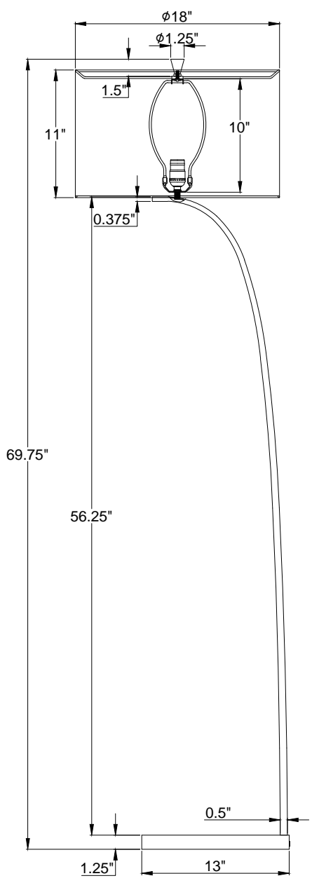
FRONT VIEW
