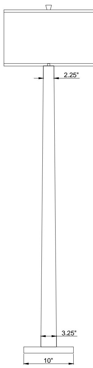
SIDE VIEW
