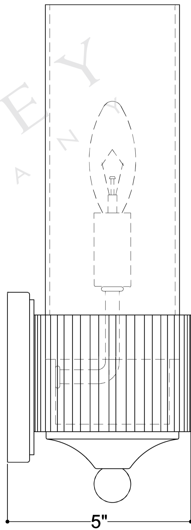
SIDE VIEW
