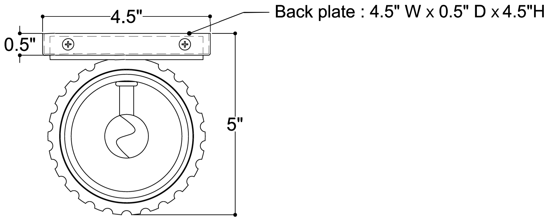
TOP VIEW
