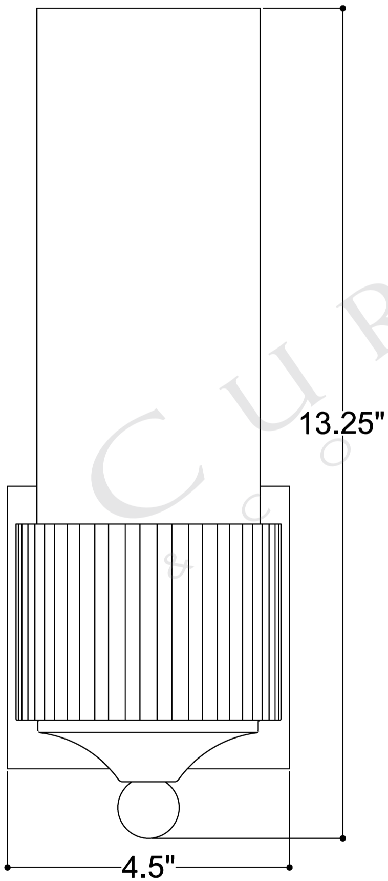
FRONT VIEW
