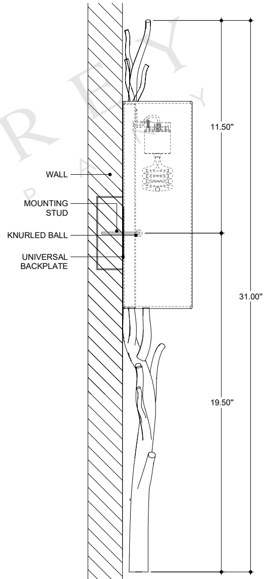
SIDE VIEW
